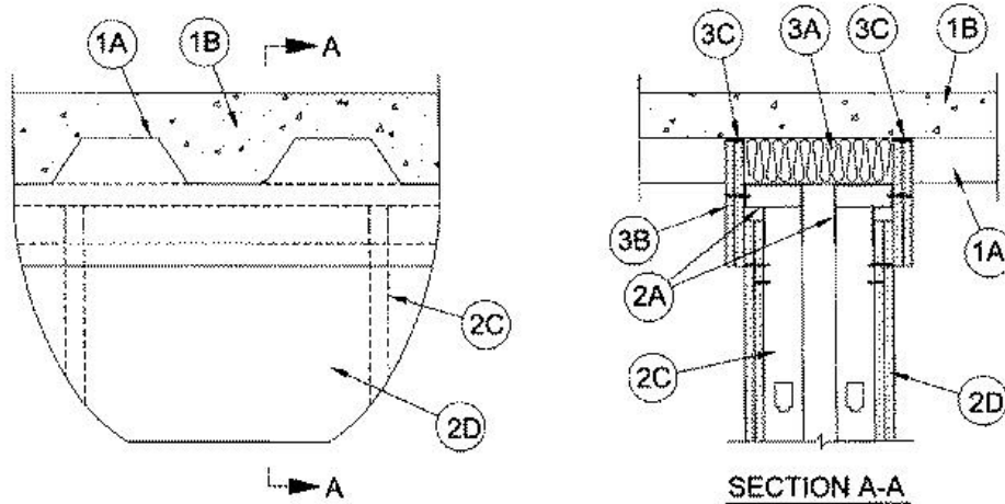
CONFIGURATION A
