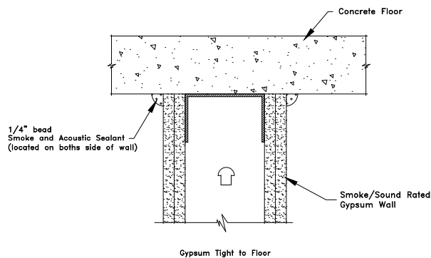
3 - 5 STC rating 62 L rating > 1 cfm cu. ft.
