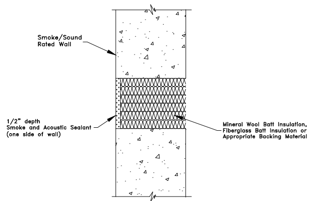
4 - 6 STC rating 62 L rating > 1 cfm cu. ft.
