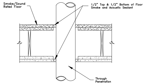
4 - 4 STC rating 62 L rating > 1 cfm cu. ft.
