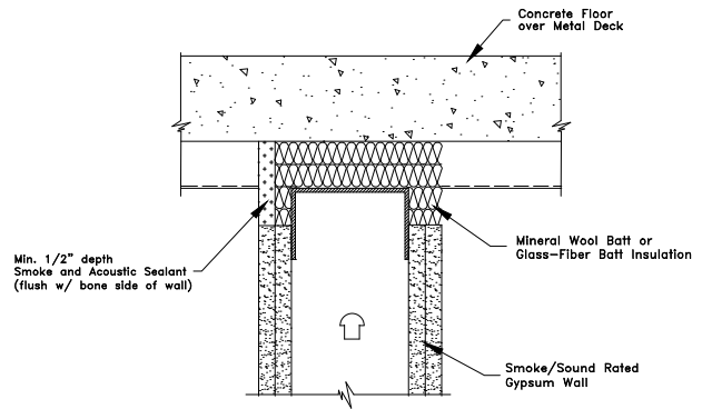
3 - 2 STC rating 62 L rating > 1 cfm cu. ft.
