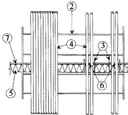
SECTION G-G
