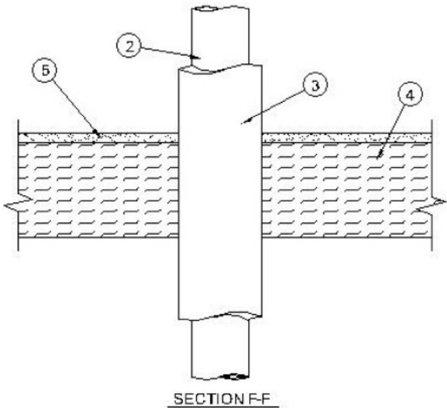
FIRESTOP CONFIGURATION F
