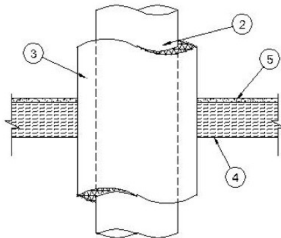
SECTION H-H
