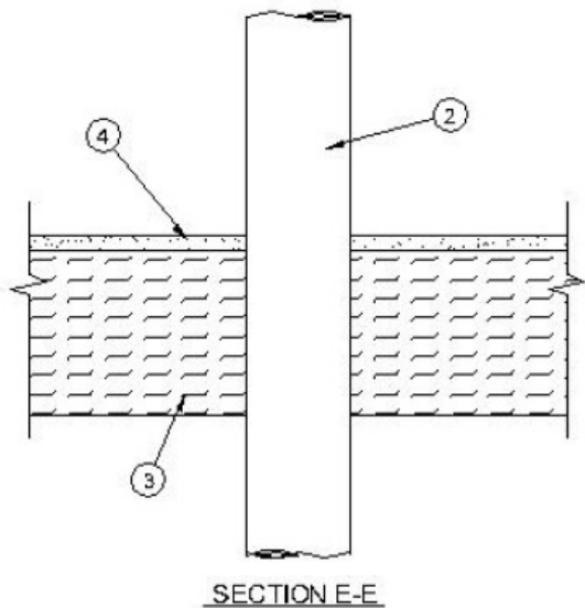
FIRESTOP CONFIGURATION E
